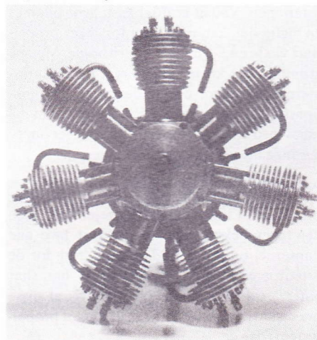
7-cylindret Deofok 1940-45
